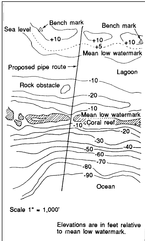
Figure 3-2. Hydrographic survey
